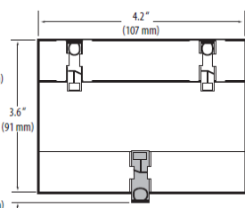
Mounting diagram
