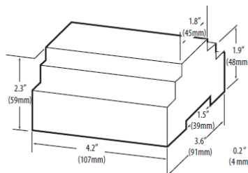
Dimensional diagram
