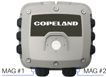
Figure 4-1 - Magnetic Switches
