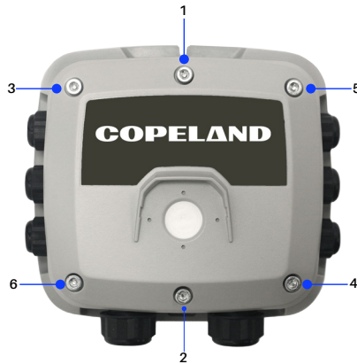
Figure 5-4 - Tightening Pattern
