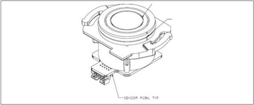
Figure 5-2 - MRLDS-450 Components
