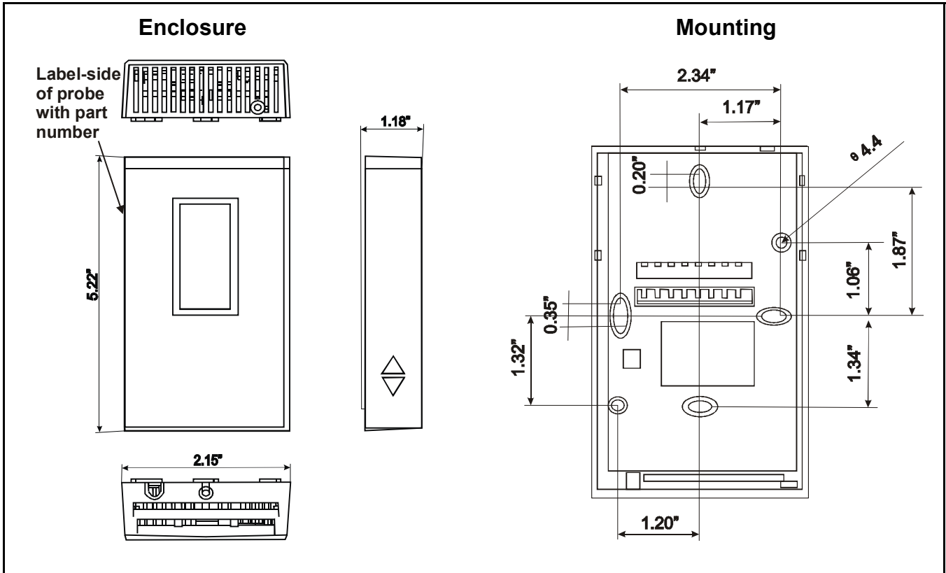
Figure 1 - Enclosure Dimensions and Mounting Plate
