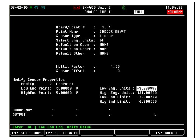
Figure 5 - E2 Input Setup
