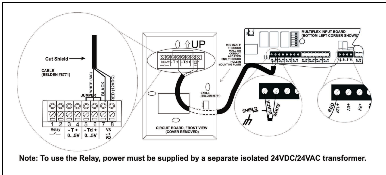
Figure 3 - Dewpoint Probe Wiring
