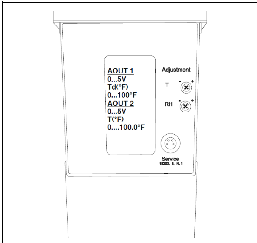
Figure 4 - HMW90 Power Up Screen
